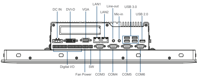
Front I/O
