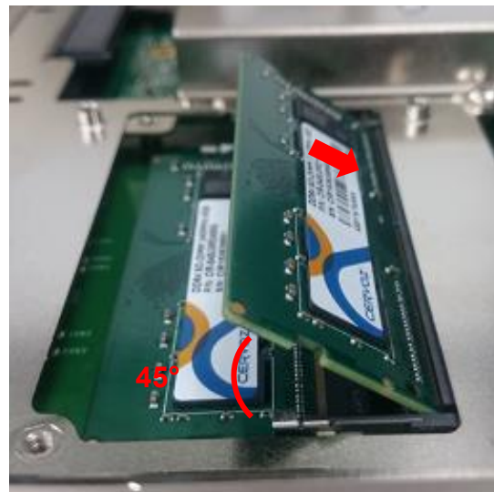
Upper socket
